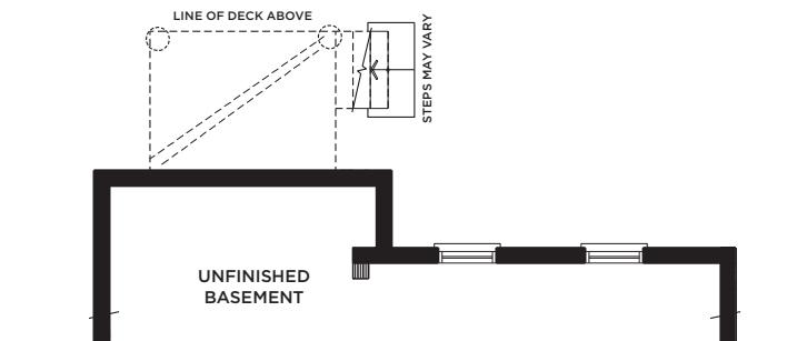
PART. BASEMENT ELEV. A & C - L.O.D. CONDITION
